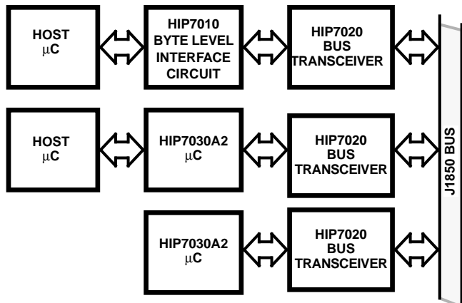
FIGURE 9. TYPICAL J1850 SYSTEM CONFIGURATIONS
