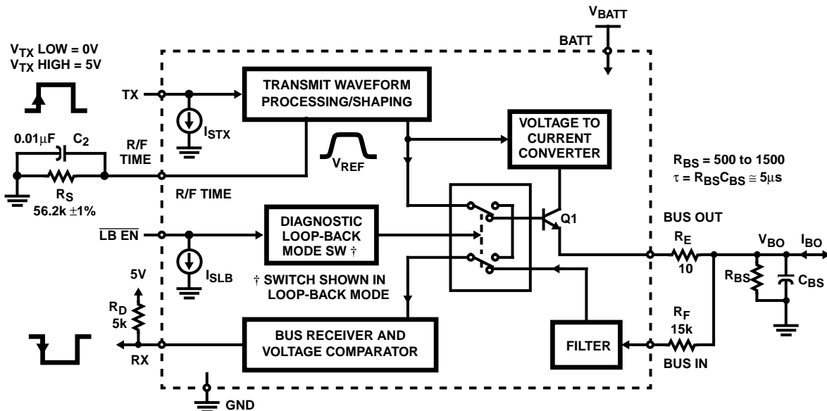
FIGURE 5. ELECTRICAL SPECIFICATION TEST CIRCUIT
