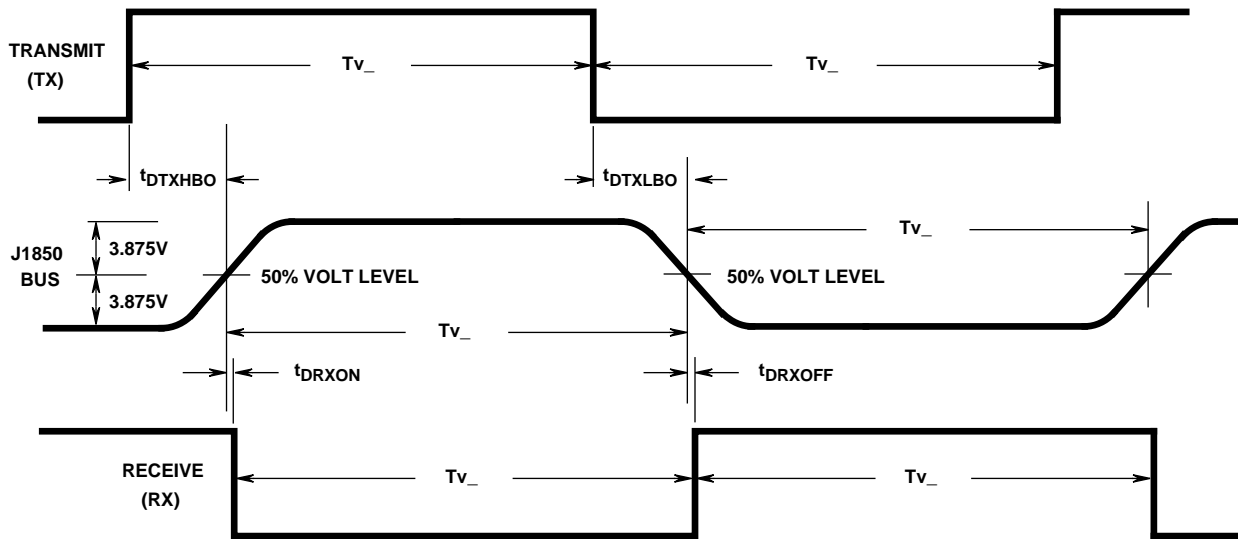
FIGURE 7. PROPAGATION TIME DELAYS
