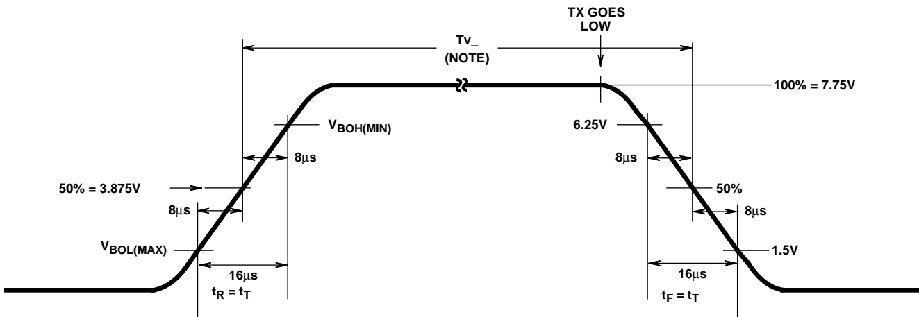
FIGURE 6. J1850 BUS WAVEFORM
