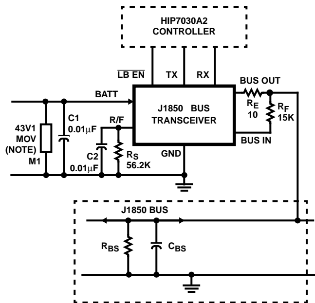
NOTE: MOV, M1 represents central protection, typically on the alternator.
