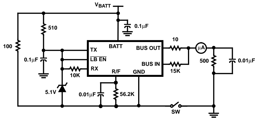
FIGURE 4. LOSS OF GROUND LEAKAGE TEST CIRCUIT
