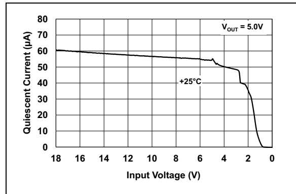
FIGURE 2-6: Quiescent Current vs. Input Voltage.
