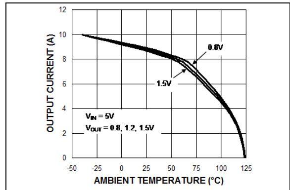
FIGURE 2-30: Thermal Derating vs. Ambient Temperature ( Note 1 ).
