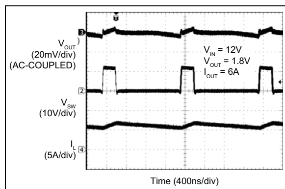
FIGURE 2-48: Switching Waveforms ( I_{OUT} = 6A ).
