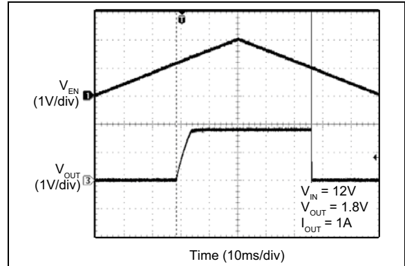
FIGURE 2-40: Enable Thresholds.
