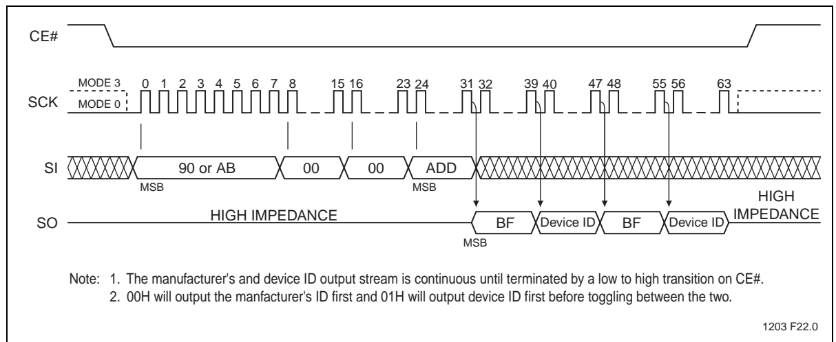
Figure 23: Read-ID Sequence
