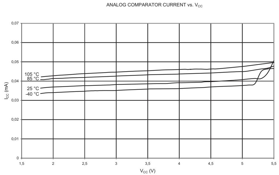
Figure 2-41. Analog Comparator Current vs. V_{CC}
