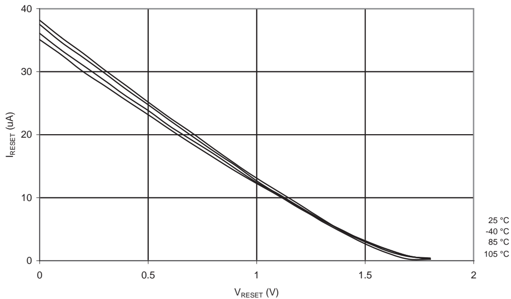
Figure 2-19. Reset Pull-up Resistor Current vs. Reset Pin Voltage ( V_{CC} = 3V )
